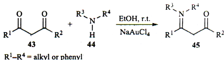
Scheme 11: Preparation of Ketimines at Room Temperature in the Presence of an NaAuCl 4 Catalyst
