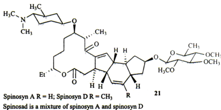
Figure 2: Chemical Structure of Spinosad – An Environmentally Friendly Insecticide
