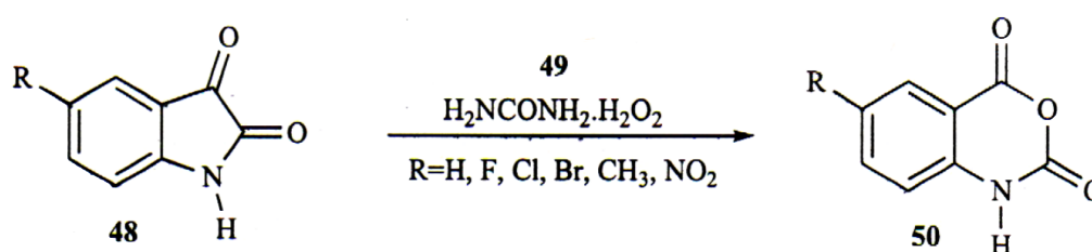
Scheme 12: Oxidation of Isatins with Urea/Hydrogen Peroxide Complex and Ultrasound Irradiation at Room Temperature
