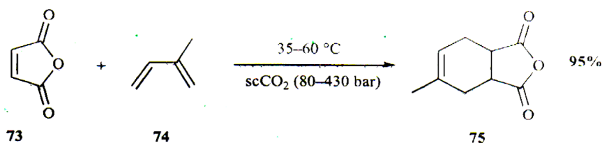
Scheme 19: Diels–Alder Reaction in scCO 2
