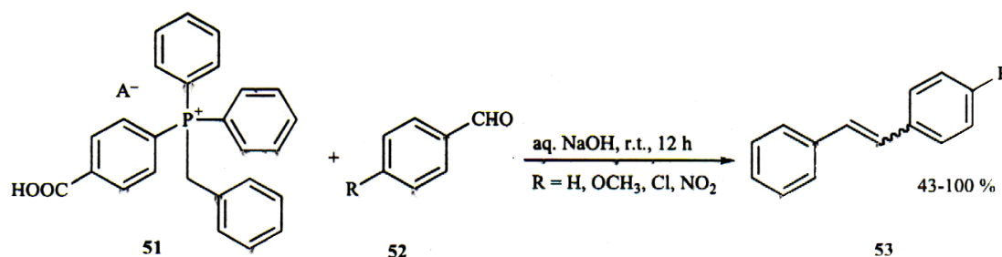
Scheme 13: Wittig Reaction in Aqueous Media
