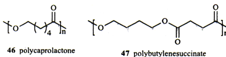
Figure 3: Chemical Structures of Biodegradable Polymers Polycaprolactone ( 46 ) and Polybutylenesuccinate ( 47 )
