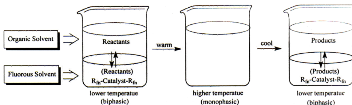
Figure 5: Schematic Representation of Organic Syntheses in Fluorinated Solvents
