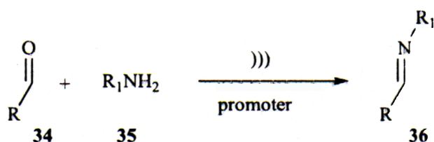
Scheme 8: Preparation of Imines using Alternative Energy Source
