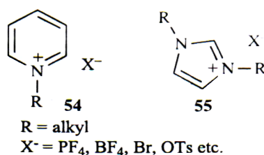
Figure 4: Chemical Structures of Some Widely used Ionic Liquids
