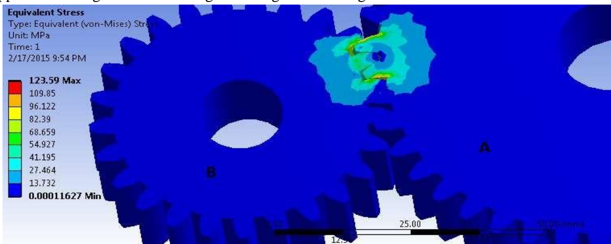
Von mises stress distribution in gear A
