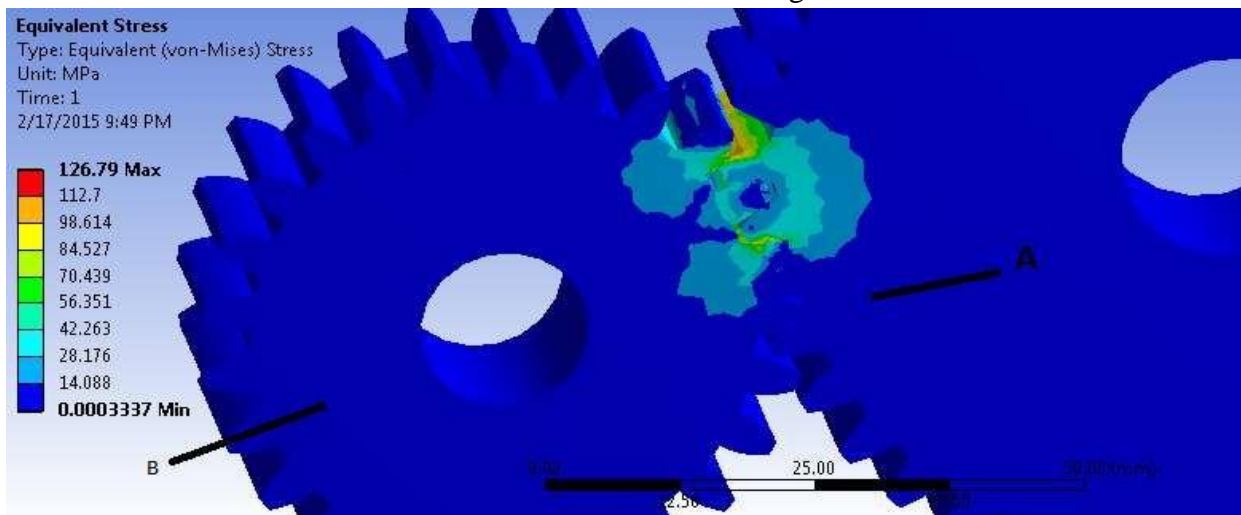
Von mises stress distribution in gear B
