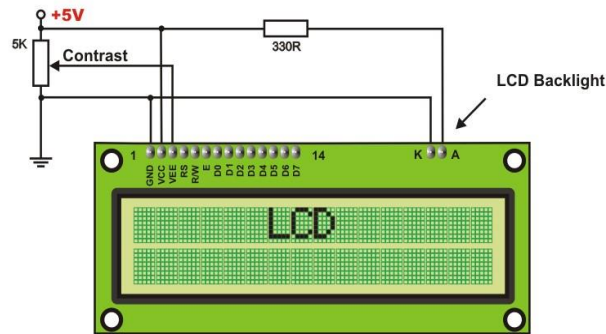
Figure: LCD Display
