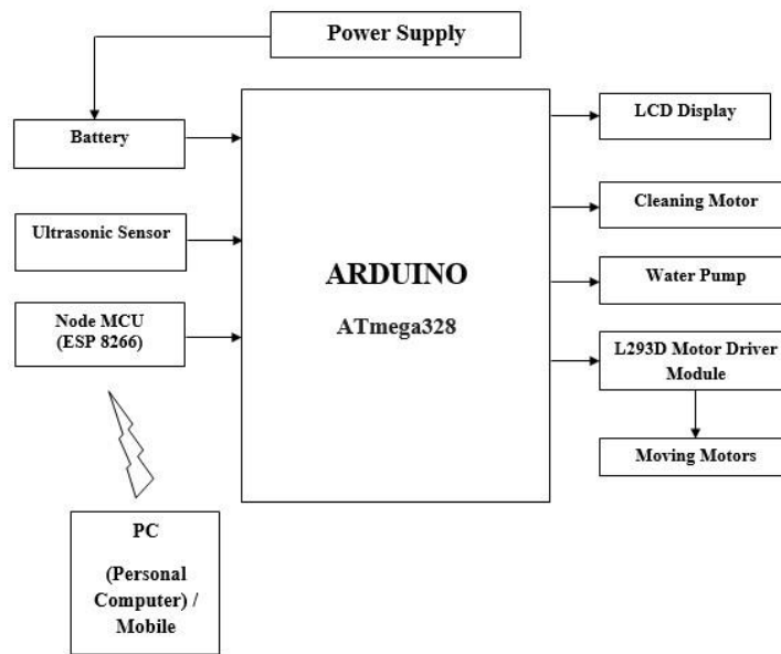
Figure: Block diagram
