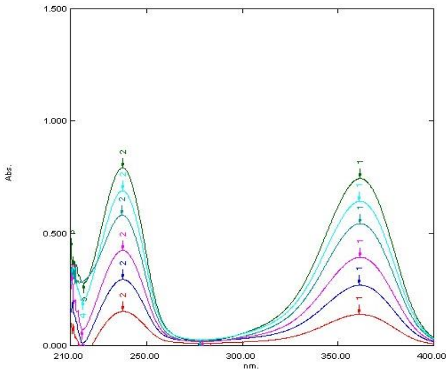
Fig.3: Area under curve overlain spectra of Favipiravir showing absorbance at 356-366nm.
