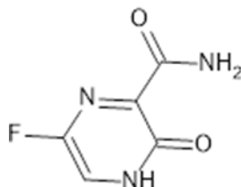
Fig.1: Chemical structure of Favipiravir
