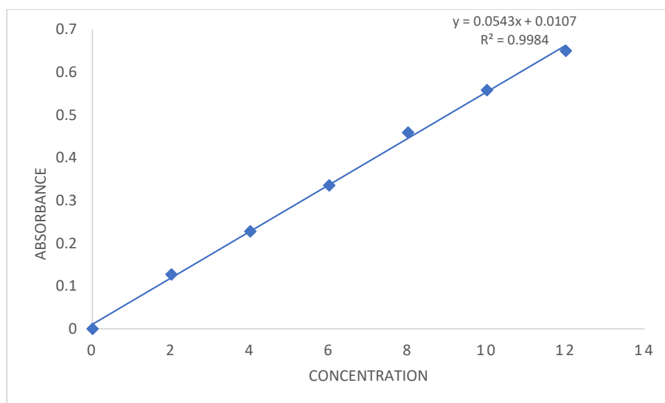
Fig.4: Calibration curve of Favipiravir at 356-366nm by Area under curve method.
