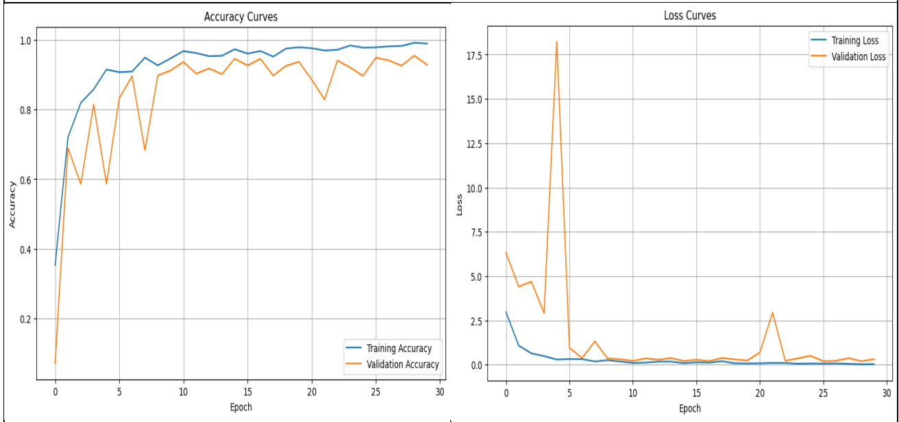
Figure 6(a): ResNet50 Graph of Accuracy Graph and Loss Curve
