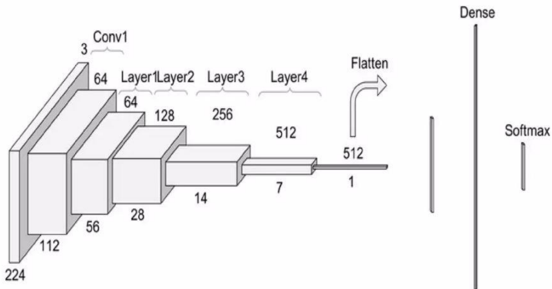
Figure 3. Diagram of ResNet 34
