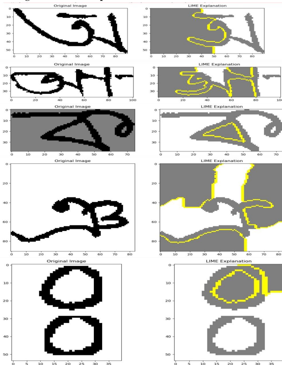
Figure 10: LIME experiment outcome on different character
