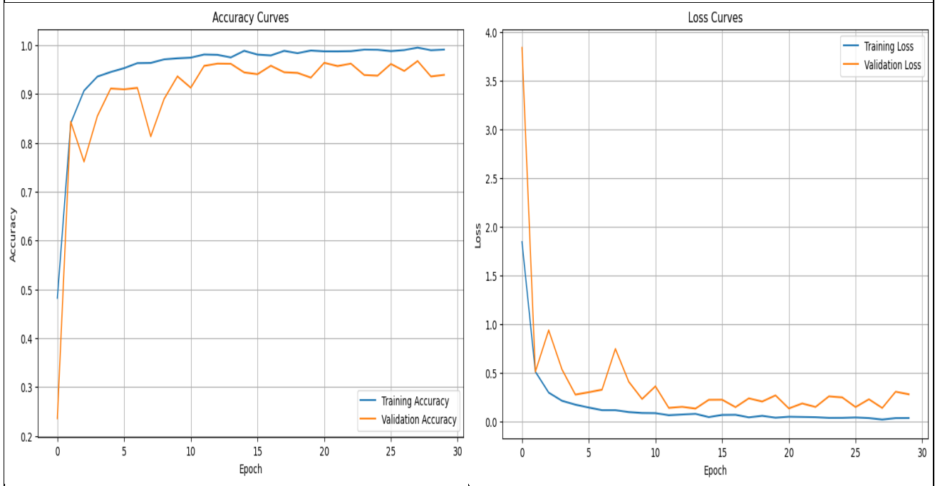
Figure 6(b): ResNet101 Accuracy Graph and Loss Curve
