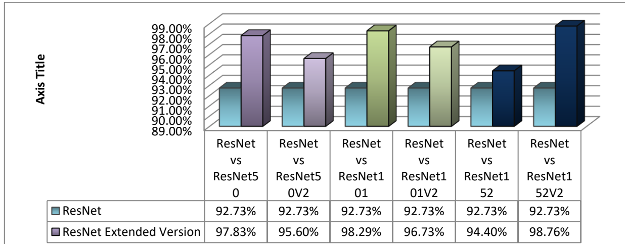
Figure 9: ResNet Vs ResNet Extended Versions Result
