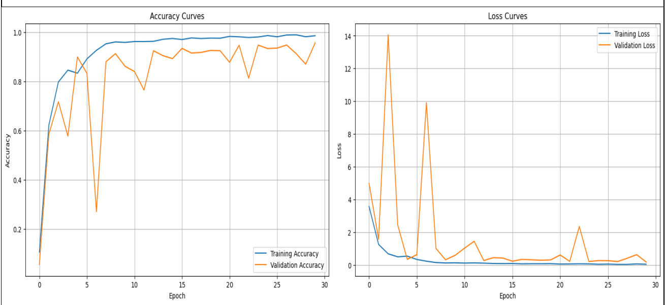
Figure 6(e): ResNet152 Accuracy Graph and Loss Curve
