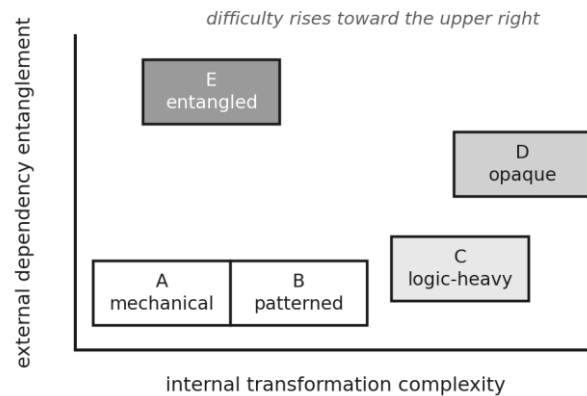
Fig. 2. Job classification. Class E difficulty arises from dependencies external to the job definition and is therefore routinely underestimated.
