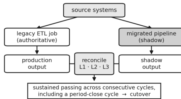
Fig. 3. Dual-run reconciliation. Legacy and migrated pipelines consume the same sources, and equivalence is established empirically before cutover.
