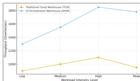
Figure 5. Throughput Performance across Workload Levels
