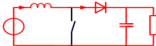
FIG 7:Operationalstates ofDC-DC Circuit
