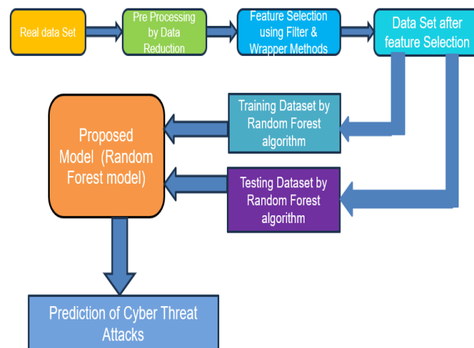
Fig 1: Overall System Architecture of Cyber Threat Detection
