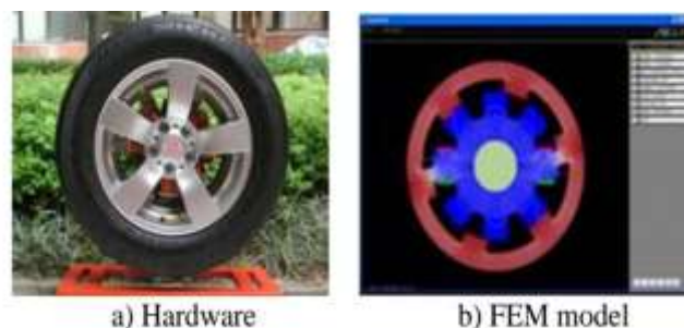
Fig 3: The in-wheel motor
