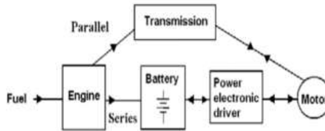
Fig 1: The series or parallel path of an HEV
