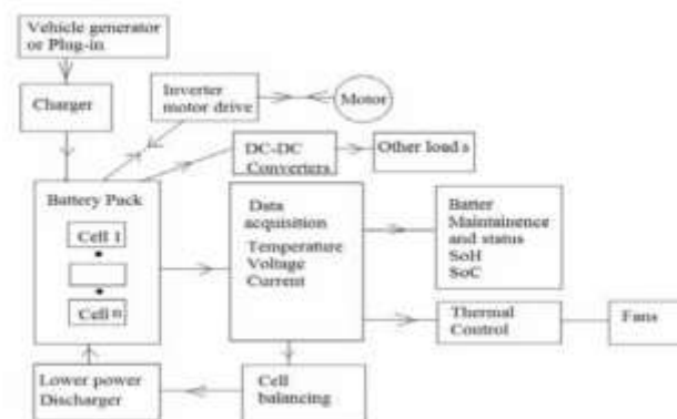
Fig 6: Schematic of the BMS 4.
