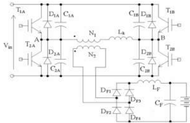
Fig 5: The H-bridge converter for charger
