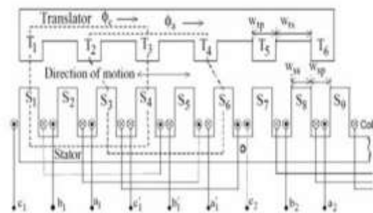
Fig 8: Active suspension based on linear motor.
