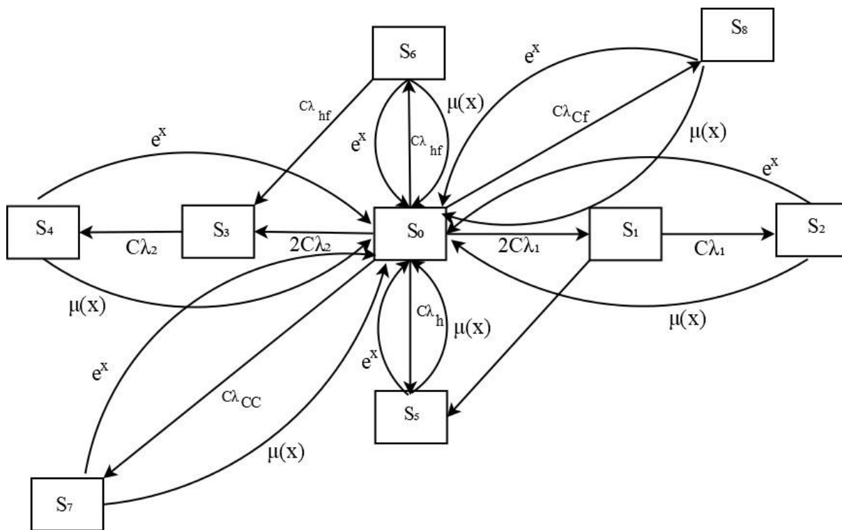
Fig 1: System Configuration
