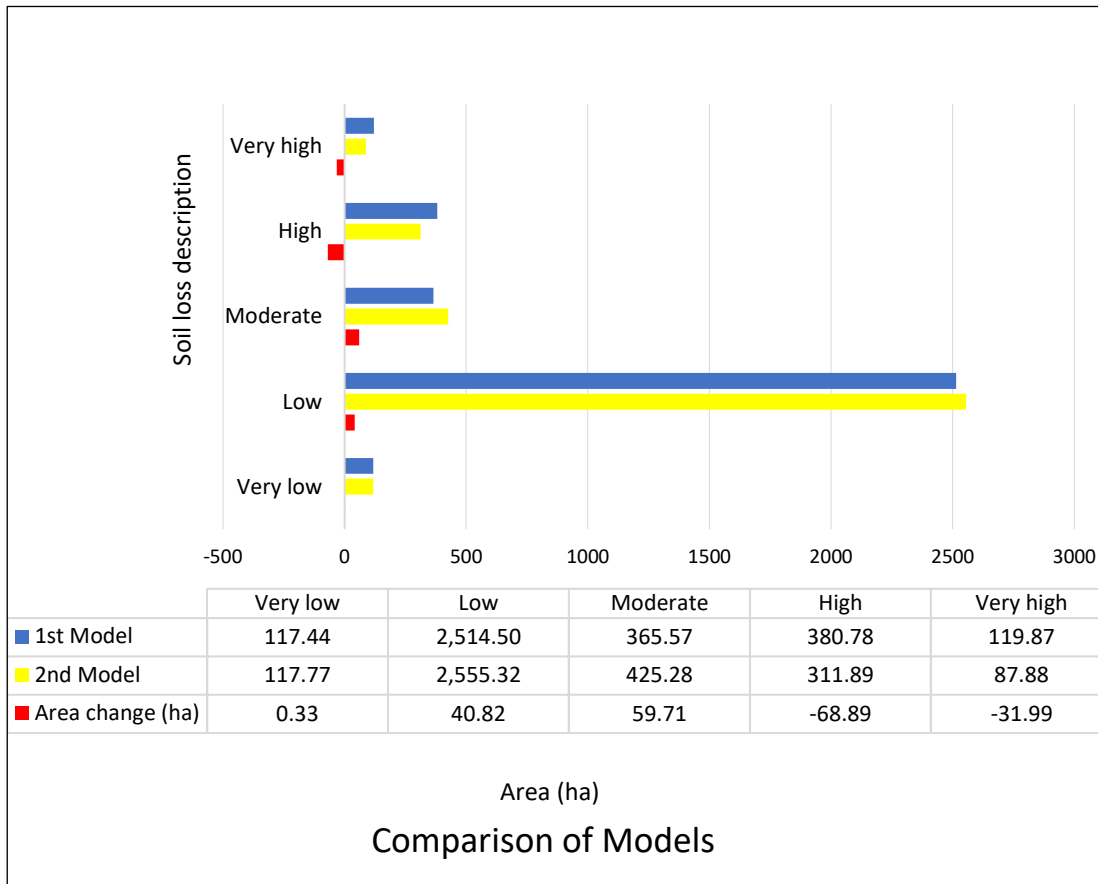
Figure 38. Visual comparison of soil loss changes showing gains and loss between the two models along the different soil loss description
