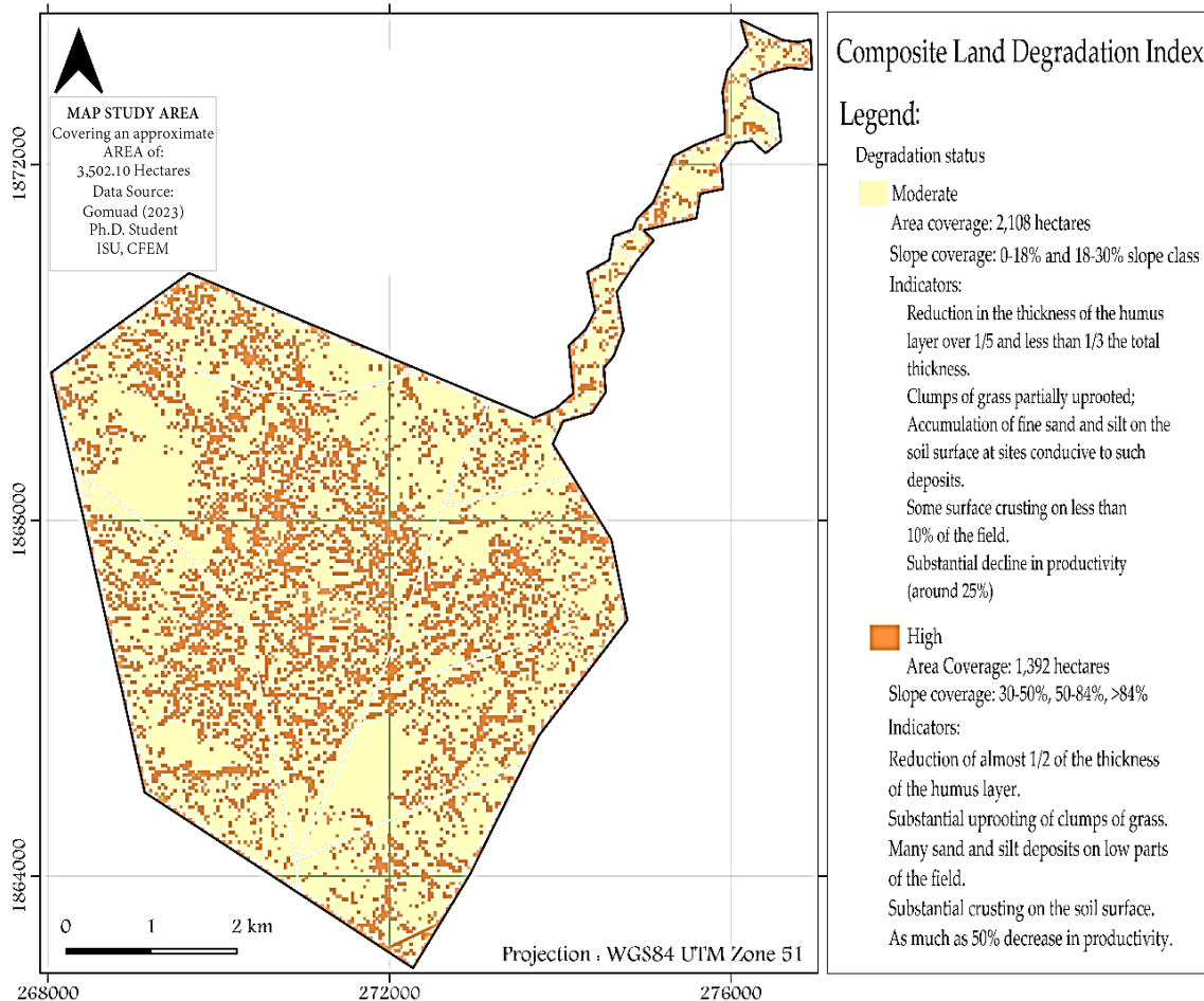
Figure 37. Map showing the composite land degradation index calculated as the sum of the degree and extent of soil erosion, with two legend colors representing moderate and high
