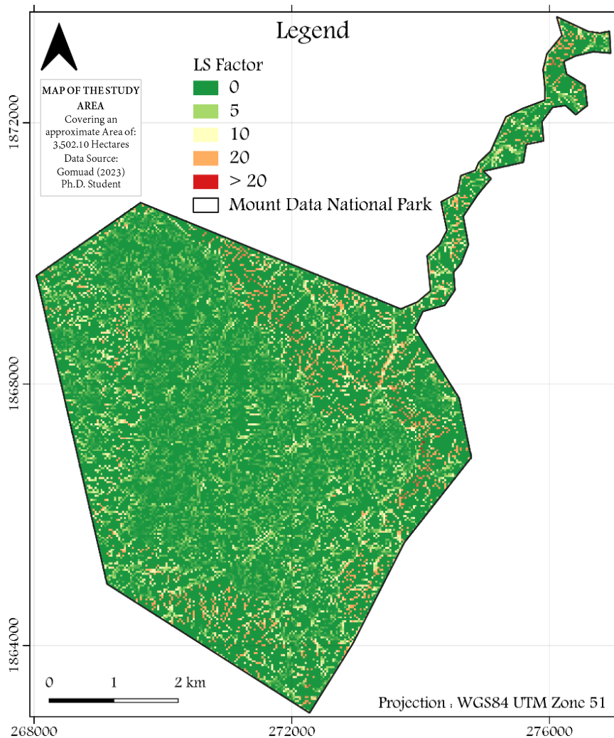
Figure 33. Map of slope length and steepness (LS) factor generated from the DEM and topographic map of the study site
