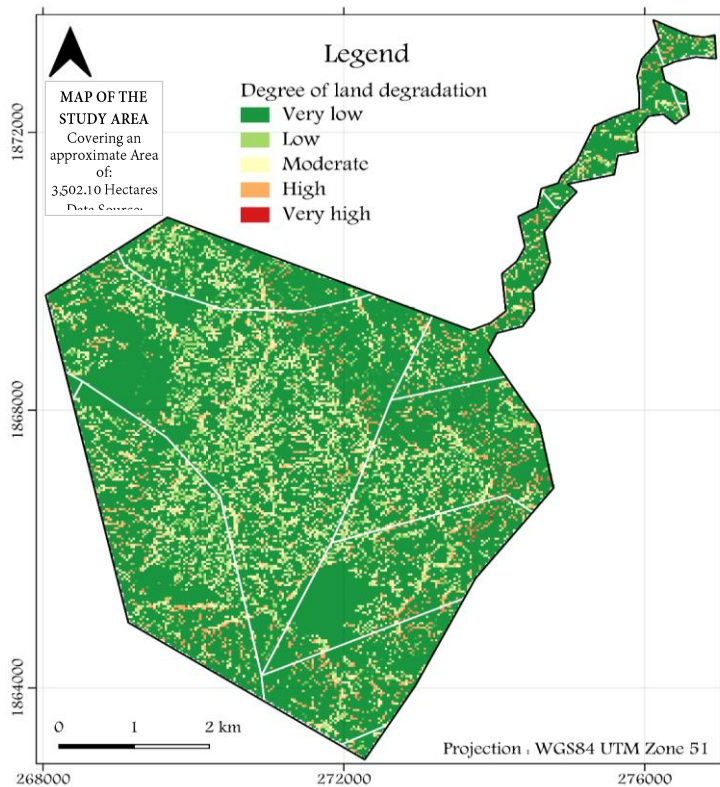
Figure 35. Map showing the annual soil loss estimates in the study area based on USLE model through Geomatics with green to red color gradient representing very low to very high erosion class
