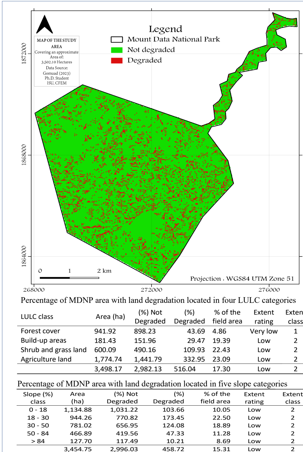
Figure 36. Map of the MDNP showing the degraded and not degraded area
