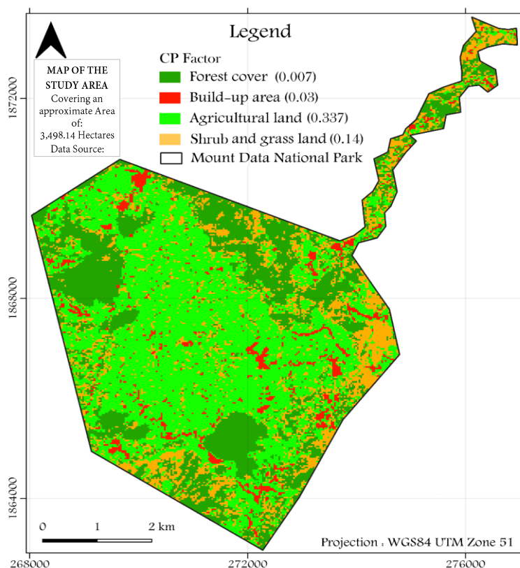
Figure 34. Map of C values quantified from land use and land cover classes adapted from the result of LULC in the earlier chapter
