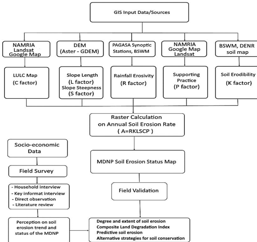
Figure 2. Sequential steps employed to estimate soil erosion by USLE Model (Modified from ARC, 1999 and BWSM, 2020)
