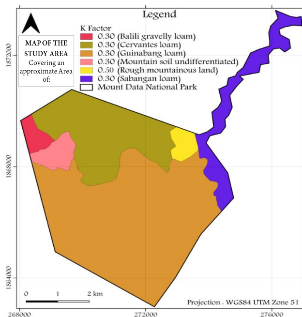
Figure 32. Soil K values map of the study site
