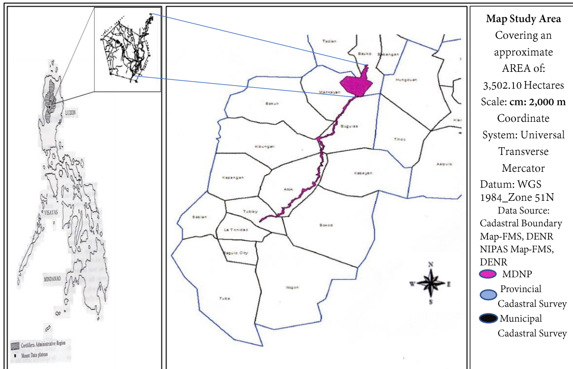
Figure 1. Location map of the Mount Data National Park
