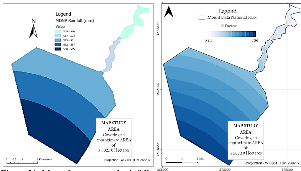
Figure 31. Map of mean annual rainfall (left) and rainfall erosivity (right) distribution of the study site
