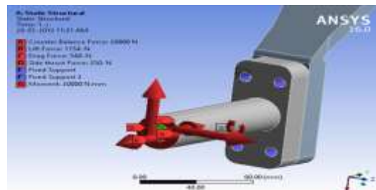
Figure 4.4 Applied loads on landing gear's leg
