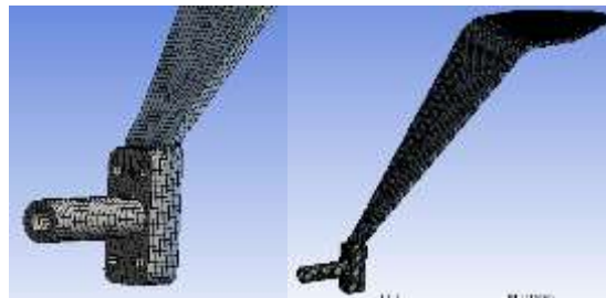
Figure 4.3 3D-Meshed model of landing gear's leg
