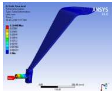
Figure 4.6 Displacement plot of the structure
