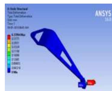
Figure 5.3 Total Deformation plot of the structure
