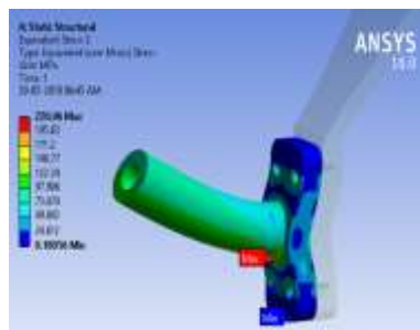
Figure 5.2 Von-Mises Stress plot of the structure
