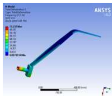
Figure Mode shape (3) at 212 Hz
