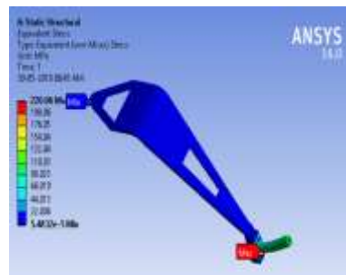
Figure 5.1 Von-Mises Stress plot of the structure
