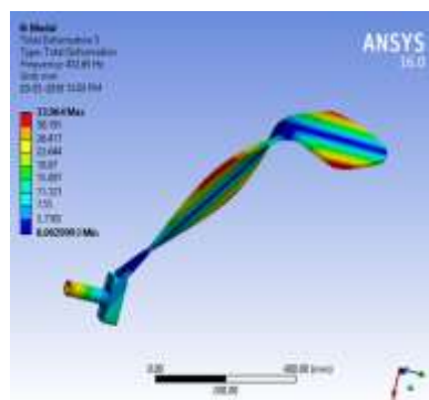
Figure Mode shape (5) at 432.65 Hz
