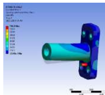
Figure 4.7 Vonmises stress plot of axle component
