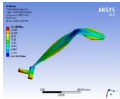
Figure Mode shape (6) at 508.75 Hz
