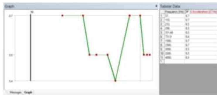
Figure 4.8 Input PSD plot of landing gear's leg
