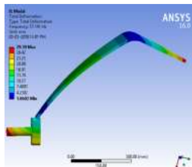
Figure Mode shape (1) at 57.141 Hz
