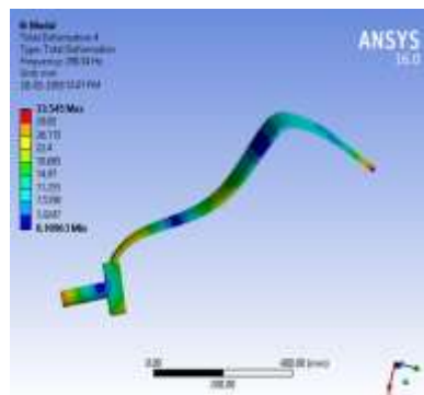
Figure Mode shape (4) at 298.34 Hz
