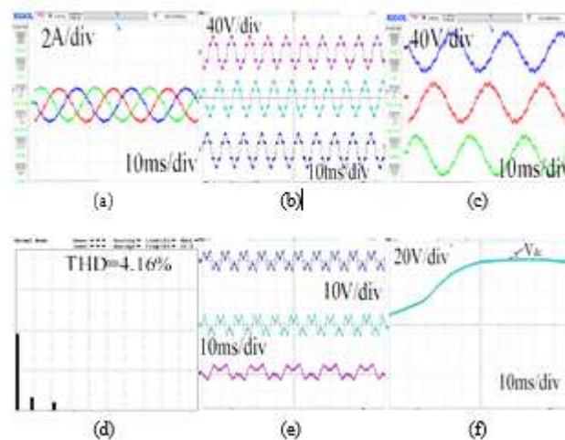
Fig. 11: Case-2a:(a) Three phase source current after compensation
