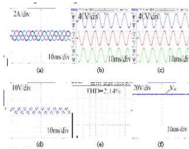
Fig. 10: Case-1b: (a) Three phase source current after compensation
