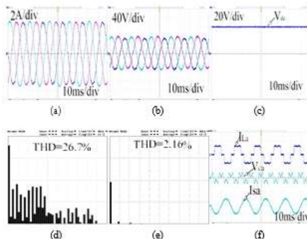
Fig. 16: Case-4b: (a) Three phase source current after compensation (b) Three phase load voltage after compensation (c) DC-link voltage (d) THD of source current before compensation (e) THD of source current after compensation (f) Compensating voltage with load current and source current after compensation in the proposed method
