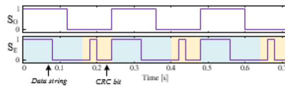
Fig. 7. S_O represents for the original 8-bit data string and S_E refers to the entire 12-bit transmitted signal.
