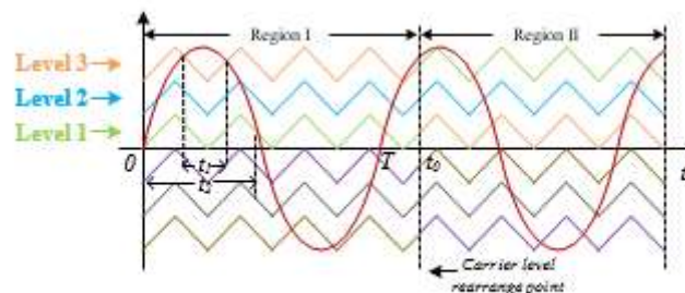
Fig. 5. Carrier level rearrangement in the PWM process.
