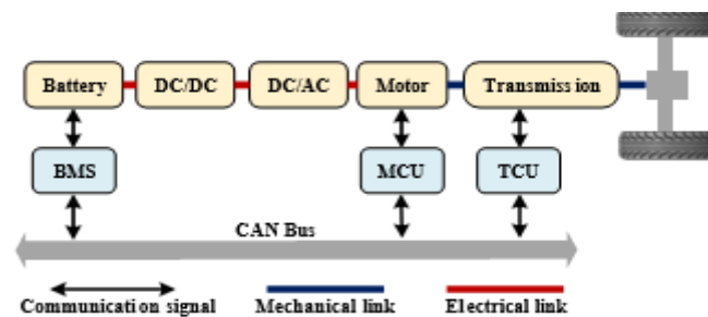
Fig. 1. The general powertrain structure of an EV
