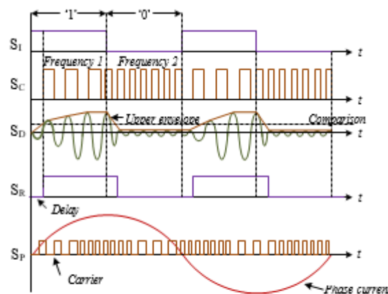
Fig. 4. The signal transmission scheme of the proposed system, where S_1 is the initial 4-bit signal '1010'; S_C is the carrier waveform; S_D represents the extracted carrier for digital '1' after using a band-pass filter; S_R shows the restored signal; S_P is the output phase current waveform superimposed with the signal's carrier.
