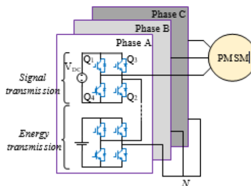
Fig. 3. Topology of the proposed P&SMT system for EVs.
