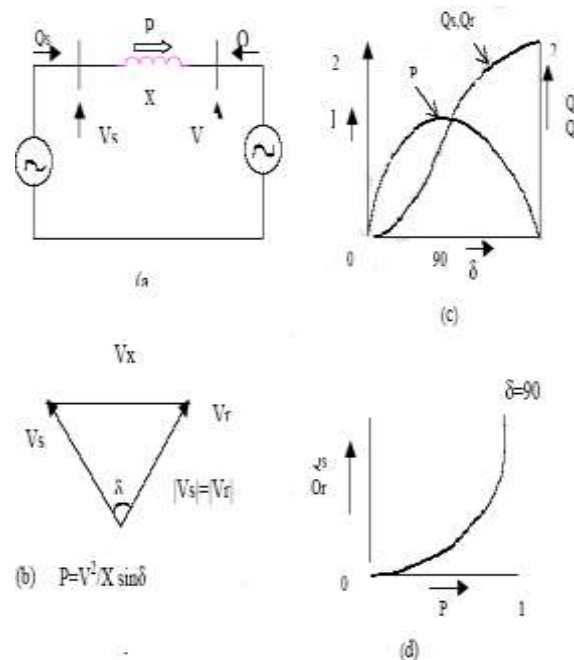
Fig.3. Simple two machine system (a) Related voltage phasor(b) Real and Reactive power verses transmission angle(c) sending end /receiving end reactive power v/s transmitted real power.
