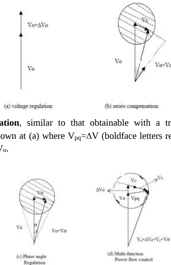
Fig.2. Basic UPFC Control Functions: a) Voltage Regulate, B) Series Compensation, C) Angle Regulation And D) Multifunction Power.
