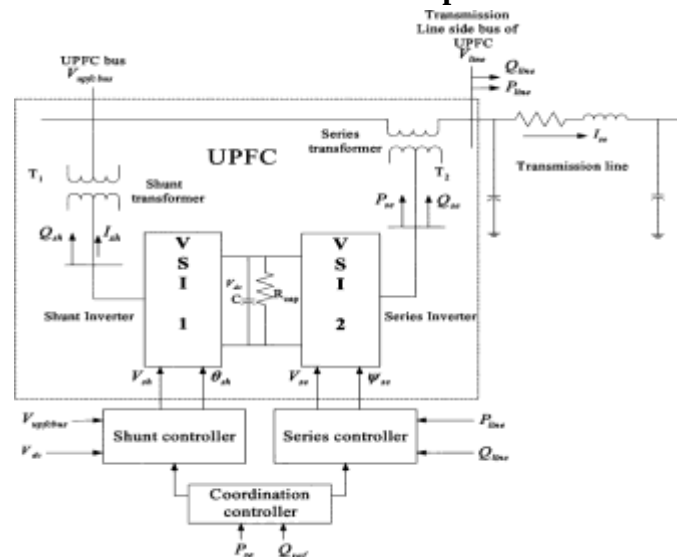
Fig.7. UPFC connected to a transmission line.
