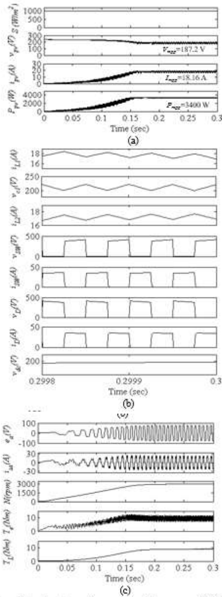
Fig. 4 Starting and steady state performances of the proposed SPV array based Zeta converter fed BLDC motor drive for water pump (a) SPV array variables, (b) Zeta converter variables, and (c) BLDC motor-pump variables.
