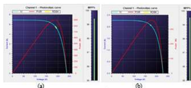
Fig. 7 MPPT performance at (a) 1000 W/m 2 , (b) 400 W/m 2
