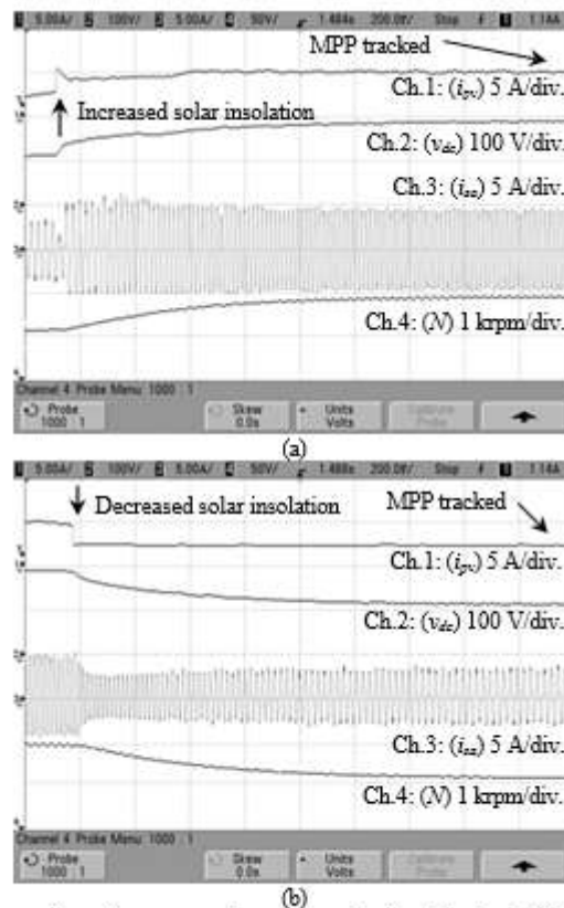
Fig.9 Dynamic performance under varying solar insolation level (a) 400 W/m 2 to 1000 W/m 2 , (b) 1000 W/m 2 to 400 W/m 2
