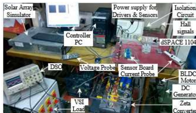
Fig. 6 Photograph of a developed prototype of the proposed system.
