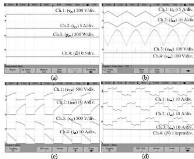
Fig. 8 Steady state performance of (a) SPV array, (b) - (c) zeta converter, (d) BLDC motor, at 1000 W/m 2
