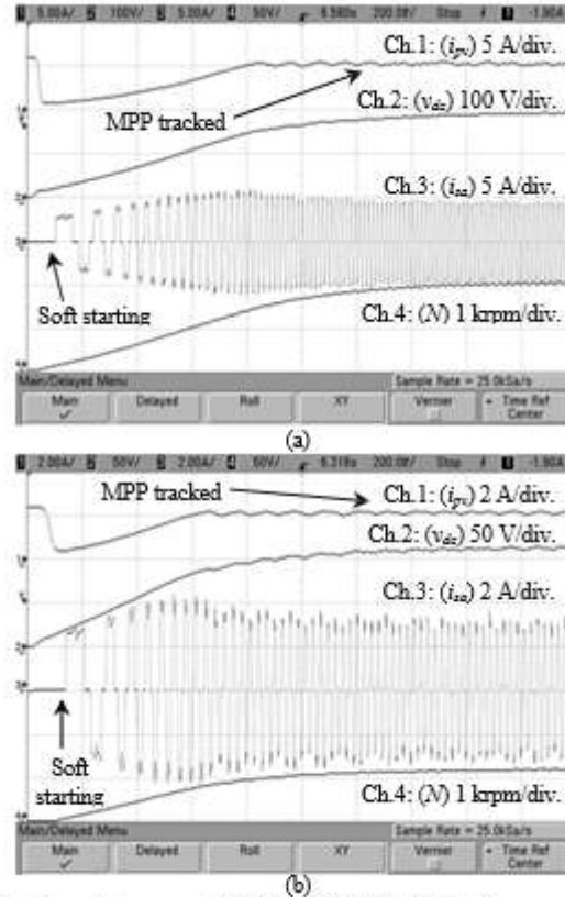
Fig.10 Starting performance at (a) 1000 W/m 2 , (b) 400 W/m 2
