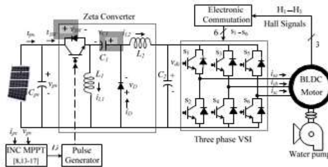
Fig. 2 Proposed SPV-Zeta converter fed BLDC motor drive for water pump.
