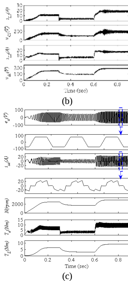
Fig. 5 Dynamic performances of the proposed SPV array based Zeta converter fed BLDC motor drive for water pump (a) SPV array variables, (b) Zeta converter variables, and (c) BLDC motor-pump variables
