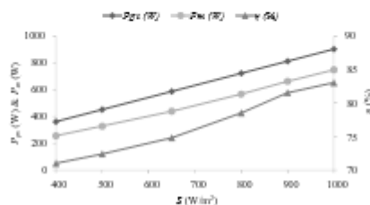
Fig. 11 Efficiency and power with solar insolation level
