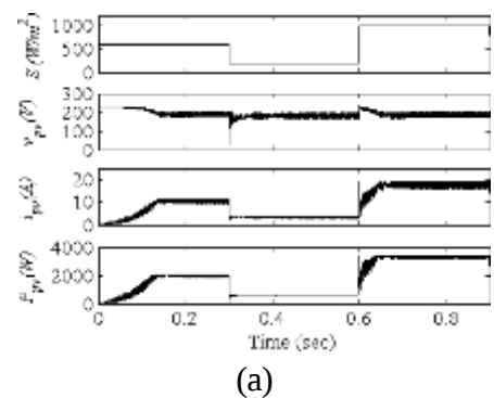
Fig. 4 Starting and steady state performances of the proposed SPV array based Zeta converter fed BLDC motor drive for water pump (a) SPV array variables, (b) Zeta converter variables, and (c) BLDC motor-pump variables.
